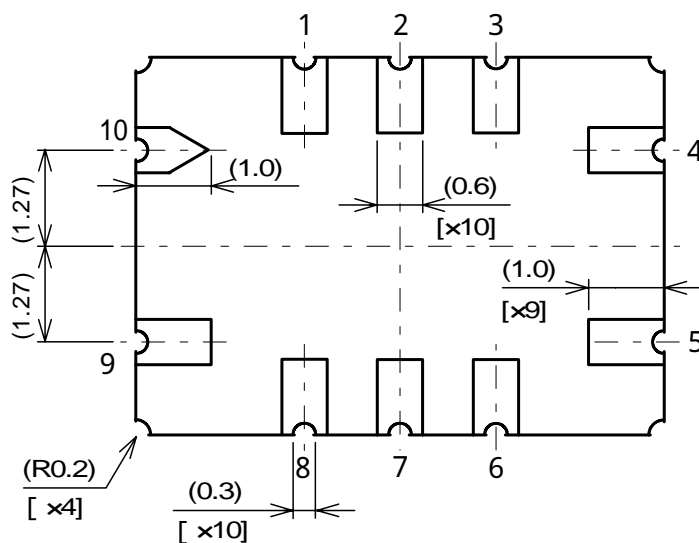
Fig.2 Package dimensions
