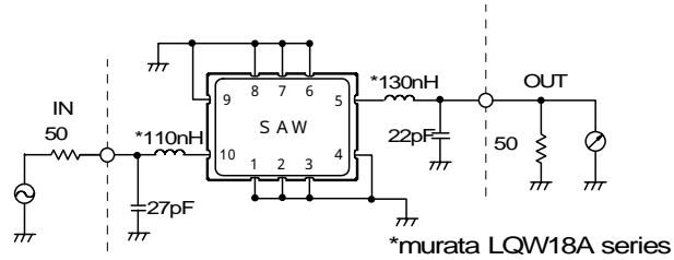
Fig.1 Measuring circuit
